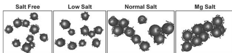
FIGURE 4 Snapshots showing distribution of the NCP particles at the end of the four coarse-grained MD simulations with different concentration of K^+ (three pictures to the left) and in the presence of Mg^{2+} (right).
